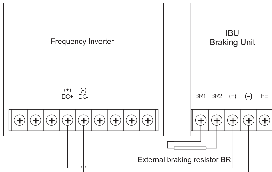
Wiring diagram of the main circuit of IBU braking unit with any kind frequency inverter
