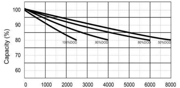
Cycle life with DOD@0.5C, 25°C
