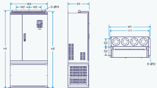
350-500kW Floor mounting Installation diagram
