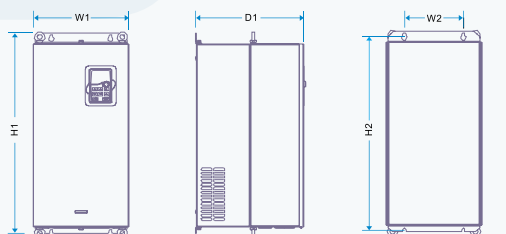
18.5-55kW Installation
