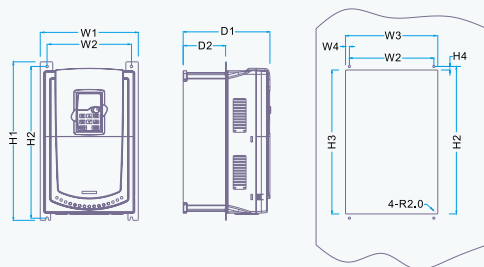
37-110kW Flange mounting Installation diagram
