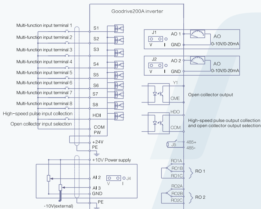
Wiring diagram of the control board
