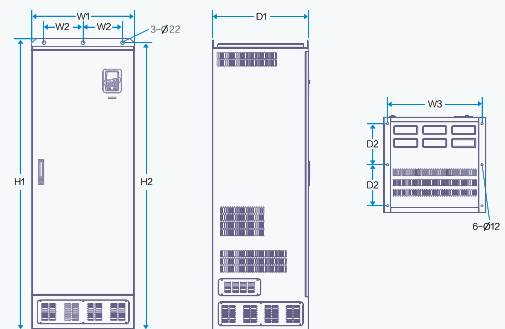
350-500kW Floor mounting Installation diagram
