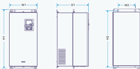
132-200kW Flange mounting Installation diagram
